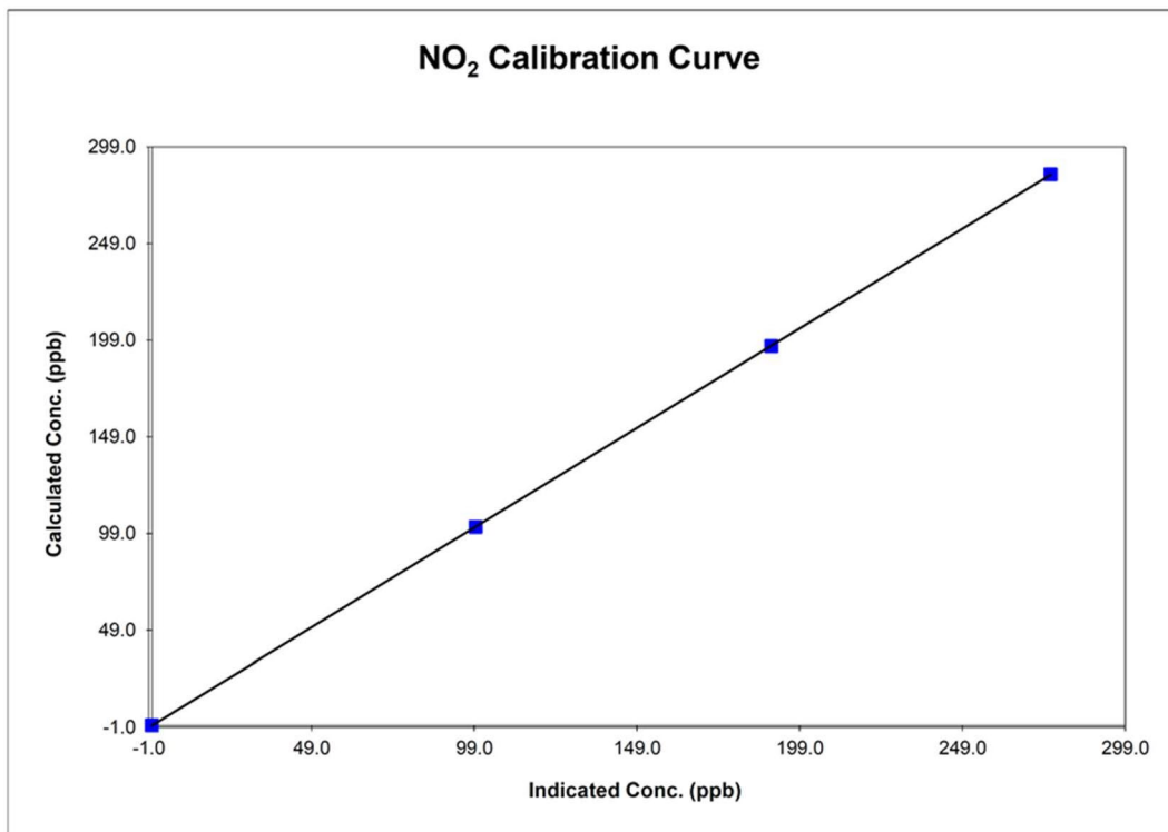
Figure 3: A graph showing the calibration of the PhoNO photolytic converter deployed inside a Thermo Fisher Scientific 42i NO x analyzer.
